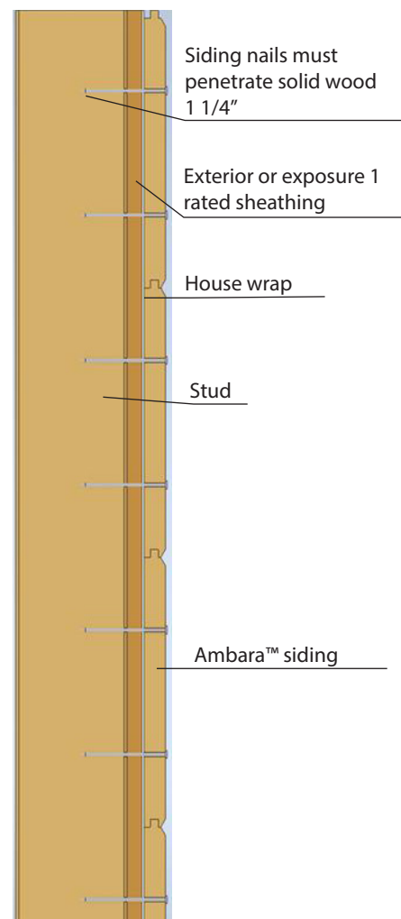
Ambara™ siding 8" or wider
